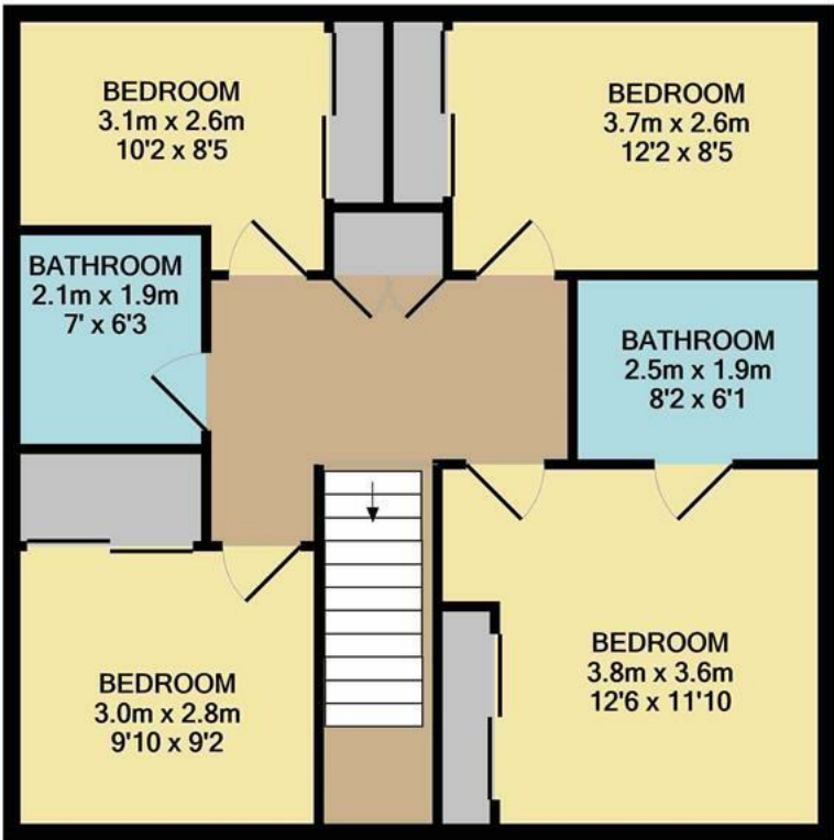
1ST FLOOR APPROX. FLOOR AREA 63.8 SQ.M. (686 SQ.FT.)
