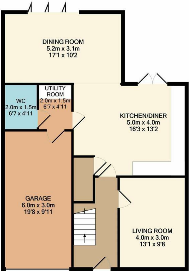
GROUND FLOOR APPROX. FLOOR AREA 79.9 SQ.M. (860 SQ.FT.)
